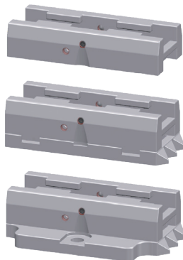
Universal mounting brackets
