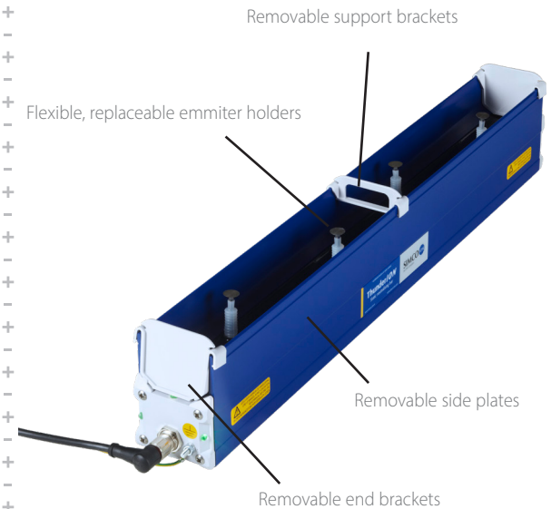
ThunderION IQ 2.0 without support -and end brackets for easy cleaning
