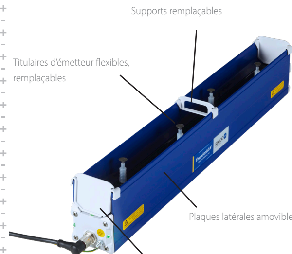
Plan ThunderION IQ 2.0
